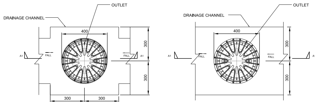
TYPE-1 LOCALISED POCKET SCUPPER DETAIL 1:10
