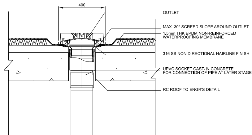
TYPE-1 LOCALISED POCKET SCUPPER DETAIL 1:10
