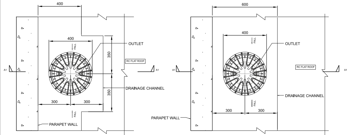
TYPE-1 LOCALISED POCKET SCUPPER DETAIL 1:10
