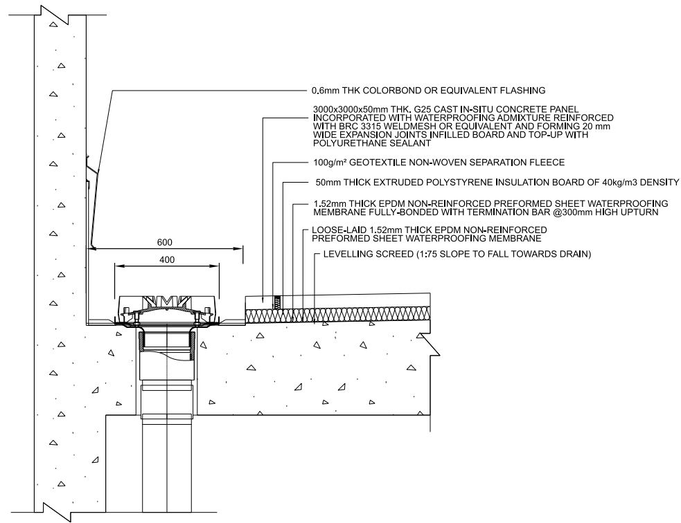
TYP. WATERPROOFING DETAIL - SECTION A1-A1 OUTLET ON RC ROOF NEAR PARAPET WALL 1:10
